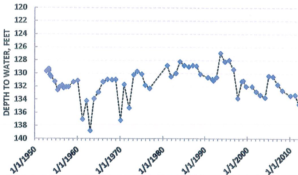
Figure 3. Hydrograph of ADWR Index Well B-17-02 06BBB.
